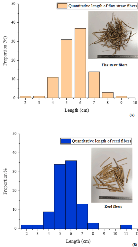
Fig. 5. Quantitative lengths of fibers: (A) flax straw and (B) reed fibers.
