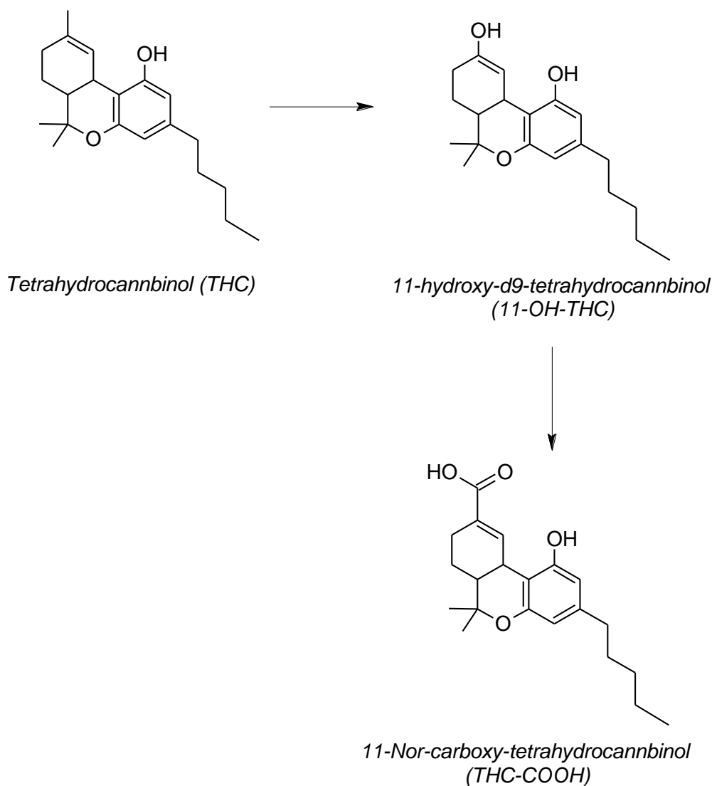
Figure 4: Metabolic route of THC to THC-COOH proposed to take place within the human body 32
