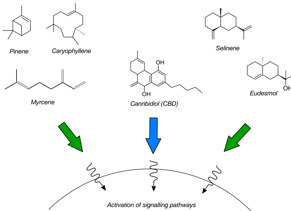
Figure 6: “The Entourage Effect” of terpenes and cannabinoids entering a cell 61 . Squiggly arrows represent the synergistic co-activating process that happen before pharmacotherapeutic effects are observed. Green arrows represent co-activating molecules, blue arrow representing CBD.
