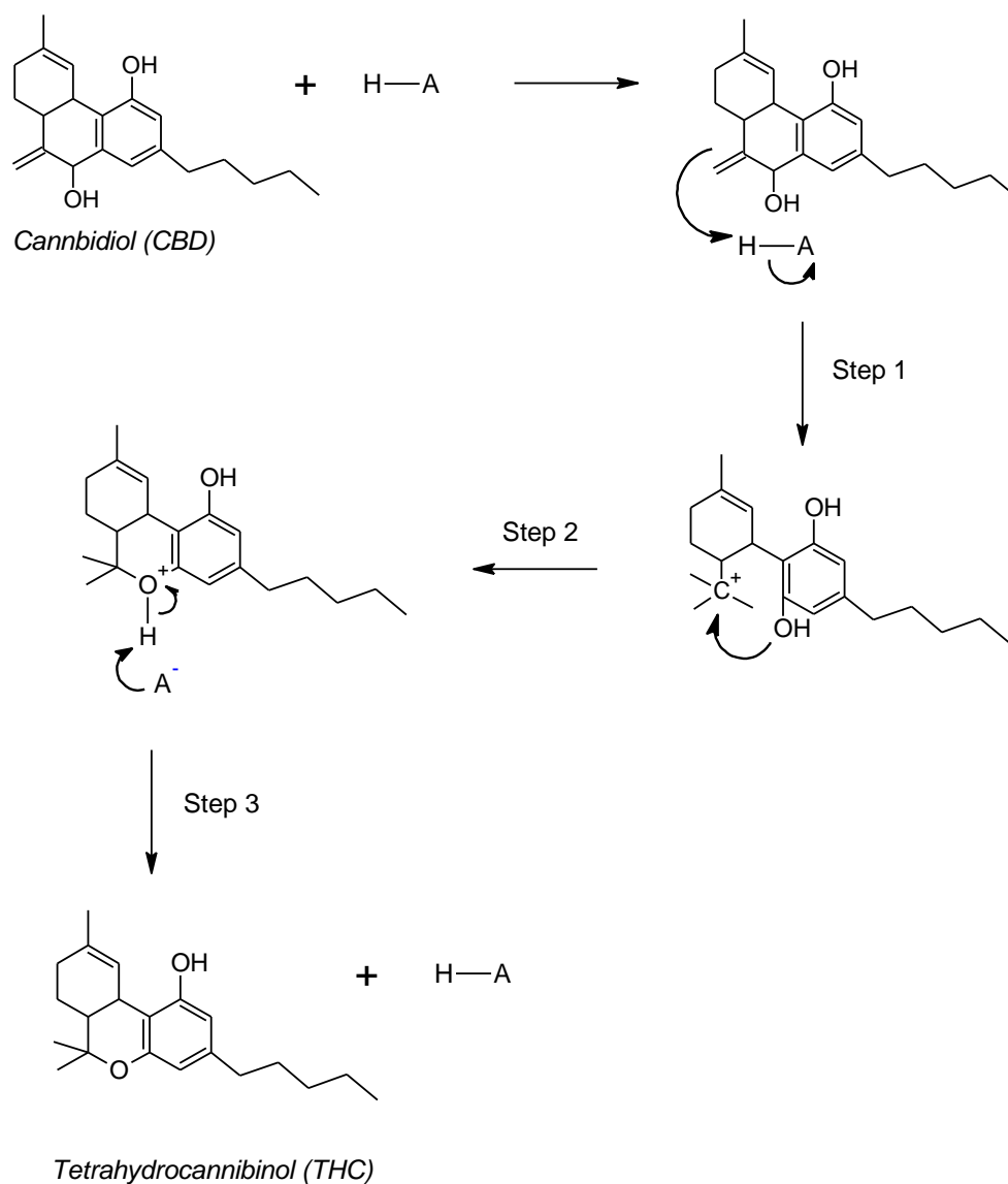
Figure 3: Acid catalyzed cyclisation reaction of CBD to THC 20
