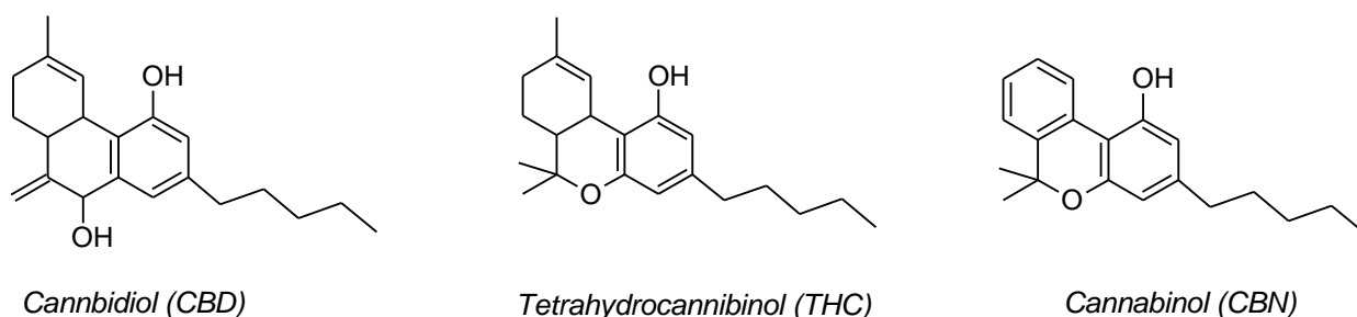
Figure 1: Structures of Cannabidiol (CBD), Tetrahydrocannabinol (THC) and Cannabinol (CBN) 1
