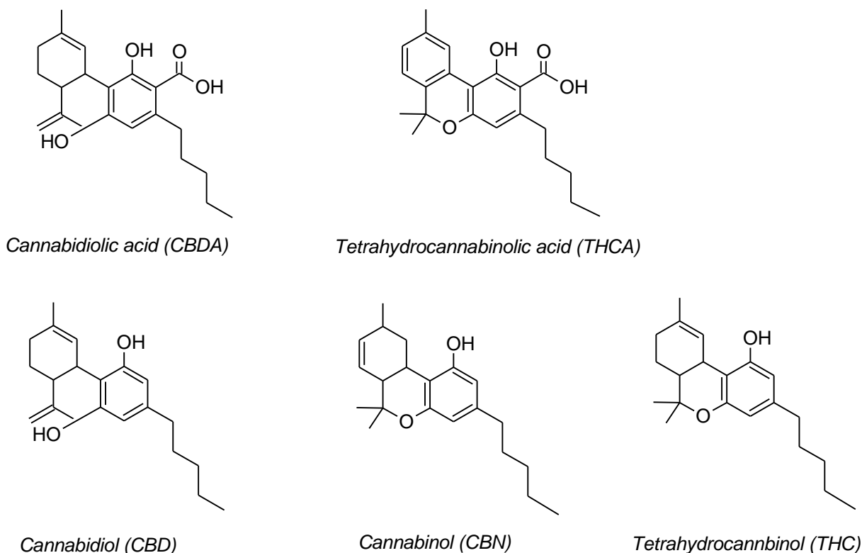
Figure 5: Cannabinoid compounds featured in analysis 1
