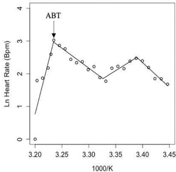
Fig. 2: Example of an Arrhenius plot, of an individual identified as Mytilus edulis with two breaks in cardiac performance. Regression lines are plotted using segmented regression analysis. Arrhenius break temperature (ABT) is shown as the final break in cardiac performance, before a rapid decline in heart rate.
