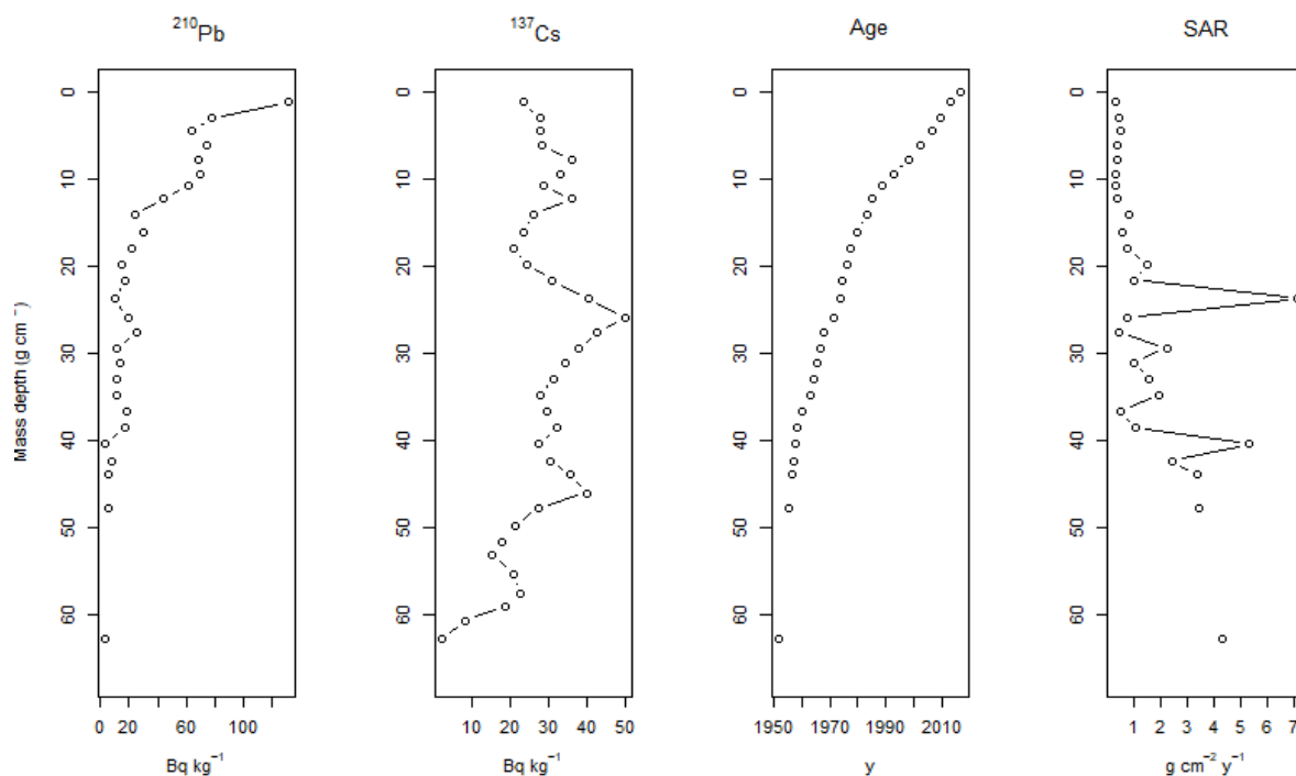
370 Figure 7: Fallout radionuclide depth profiles for (a) 210 Pb un and (b) 137 Cs with and geochronological information (c) age-depth and (d) sediment accumulation rate according to output from the Constant Rate of Supply model (see text for details).
