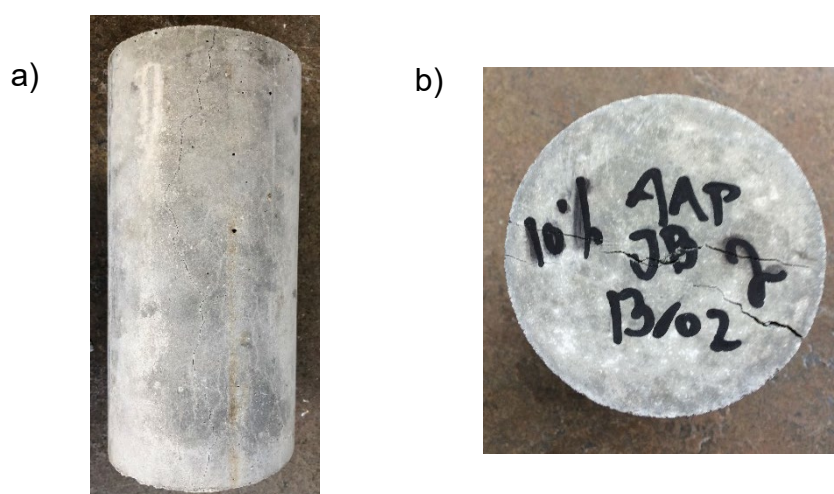
Figure 16: 150 \varnothing mm x 300 mm samples after splitting tensile failure a) 20 % replacement sample 1 b) 10 % replacement sample 2
