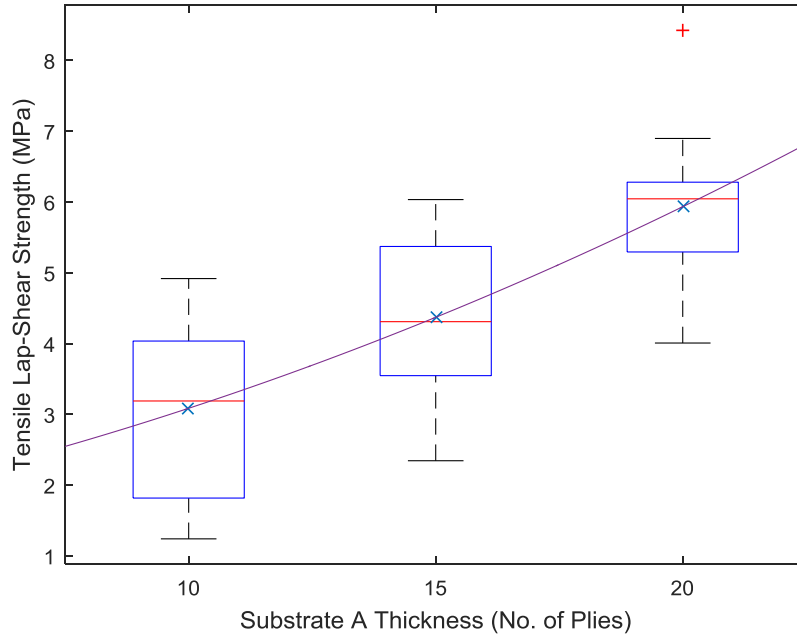
Statistical Analysis 8 - Substrate A Thickness Comparison (Adhesively Bonded)
