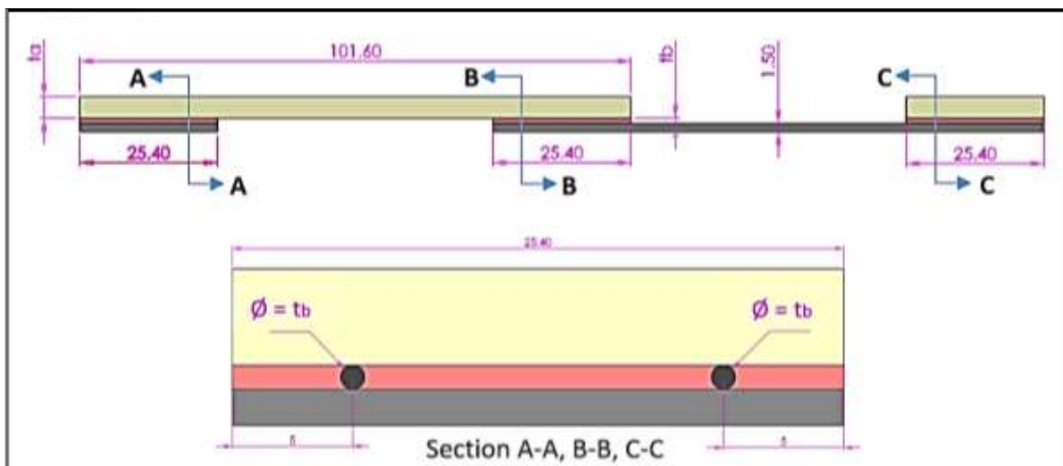
Figure 2: Specimen configuration of the adhesively bonded single-lap joints. Section view showing the cross-sectional geometry at region A-A, B-B and C-C, picturing the calibrated aluminium wire spacers which were used to control bondline thickness. (not to scale, dimensions in mm)
