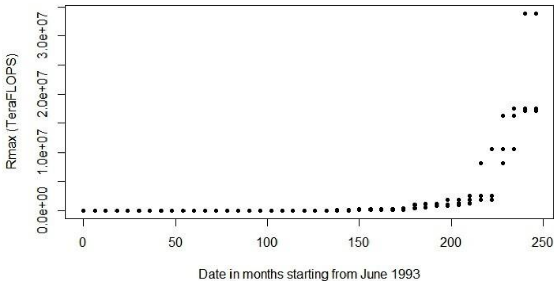
Figure 2: Plot of Rmax values for top 3 supercomputers in Top500 list since 1993.
