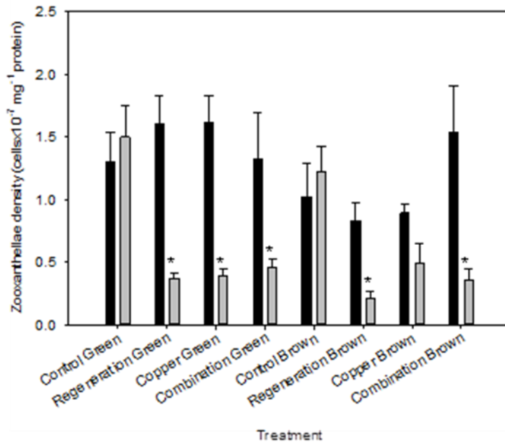
Figure 5: Zooxanthellae density before (black bars) and after (grey bars) the experiment in all treatments. Copper treatments were maintained at a concentration of 50 \mu\text{g l}^{-1} Cu. Brackets indicate standard error. Asterisks indicate significant difference as confirmed by two-way ANOVA and Holm-Sidak post-hoc test for each colour morph ( P < 0.05 , df = 3 , n = 4 )
