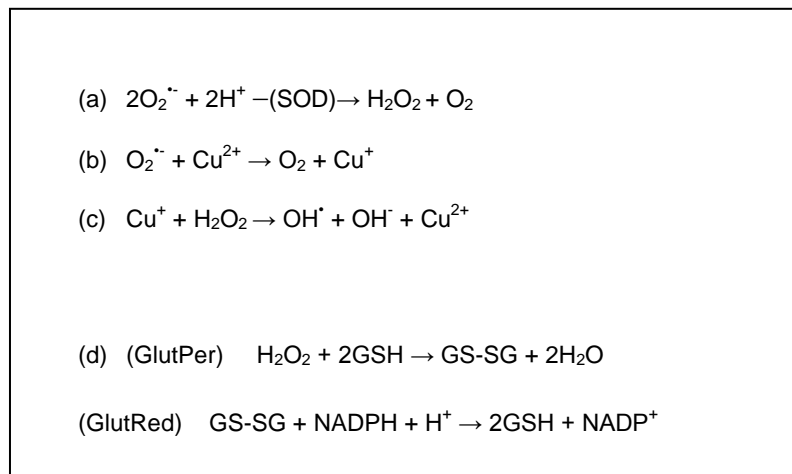
Figure 1: Copper-induced formation of reactive oxygen species and antioxidant action of glutathione. (a) Superoxide ions ( \text{O}_2^{\cdot -} ) form hydrogen peroxide ( \text{H}_2\text{O}_2 ) in a reaction catalysed by the antioxidant enzyme superoxide dismutase (SOD). (b) Copper reacts with superoxide ions and is reduced. (c) Copper donates electrons to hydrogen peroxide to form highly reactive hydroxyl radical ( \text{OH}^{\cdot} ) in the Fenton reaction (Davies, 1995; Lushchak, 2011). (d) Detoxification of hydrogen peroxide by reduced glutathione (GSH) and oxidised glutathione (GS-SG). This cyclic reaction is catalysed by antioxidant enzymes glutathione peroxidase (GlutPer) and glutathione reductase (GlutRed) and regenerates GSH for additional detoxification reactions (Halliwell & Gutteridge, 2007)
