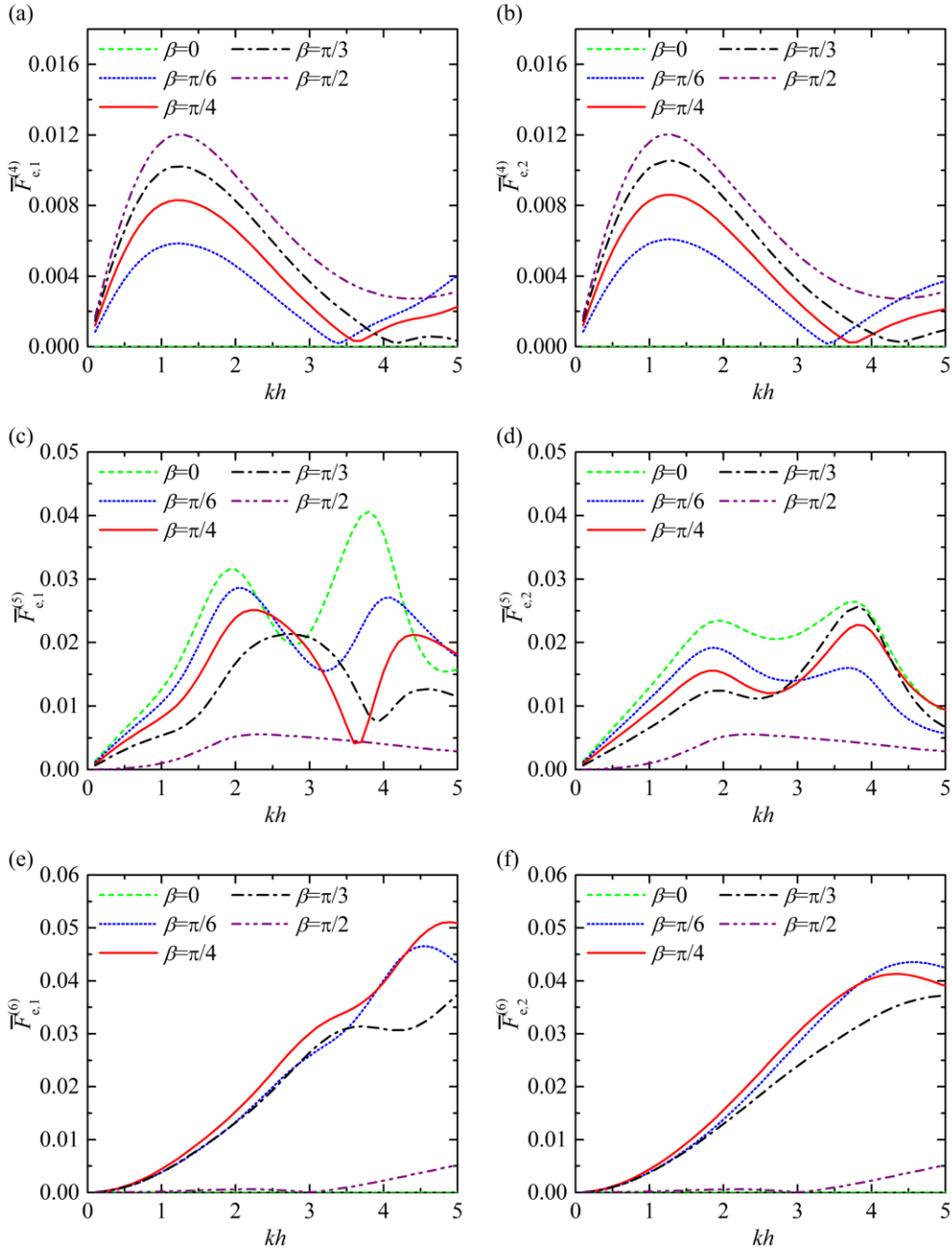
1 2 Fig. 7. Normalised wave excitation moments acting on the two caissons vs kh for five incident 3 wave angles \beta=0, \pi/6, \pi/4, \pi/3 and \pi/2 with e/h=1.0 : (a) \bar{F}_{e,1}^{(4)} ; (b) \bar{F}_{e,2}^{(4)} ; (c) \bar{F}_{e,1}^{(5)} ; (d) \bar{F}_{e,2}^{(5)} ; (e) 4 \bar{F}_{e,1}^{(6)} ; (f) \bar{F}_{e,2}^{(6)} .
